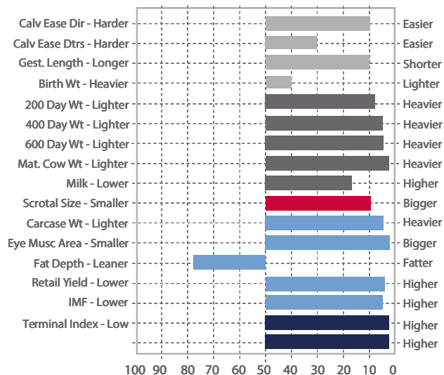
MARCH 2024 EBV PERCENTILES FOR SKAIL DALTON W214
